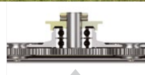
Solid bearing mounting – high level of reliability when in use
